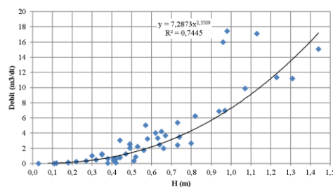
Gambar 3. Lengkung Debit Sts. Gilireng ( H \leq 1,50 m)
